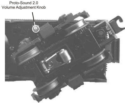
Figure 2: Manual Proto-Sound 2.0 Volume Adjustment
