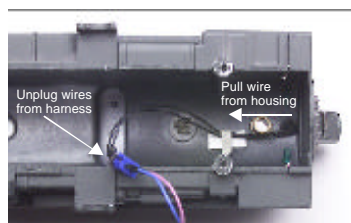
Figure 8. Replacing the Lantern Light on the Front of the Boiler
