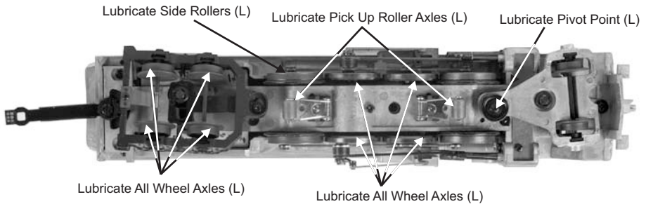
Fig. 1: Lubricating the Locomotive
