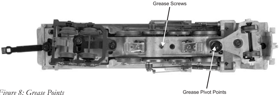
Figure 8: Grease Points
