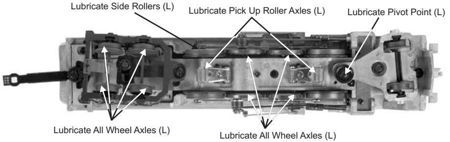
Figure 7: Lubricating the Locomotive
