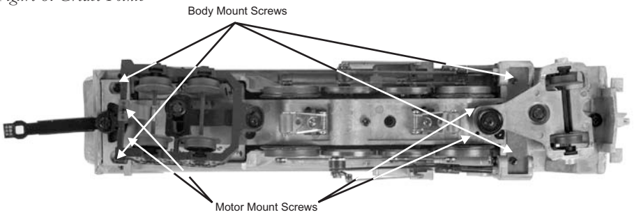
Figure 9: Body Mount Screws and Motor Mount Screws
