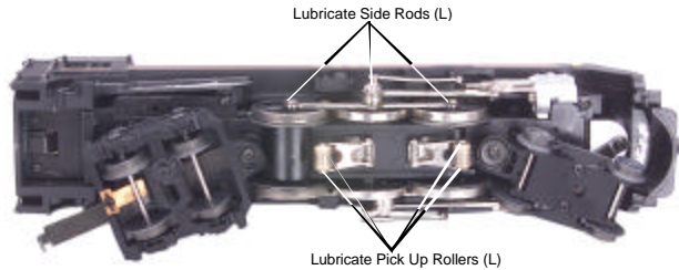
Figure 2. Lubrication Points on the Engine
