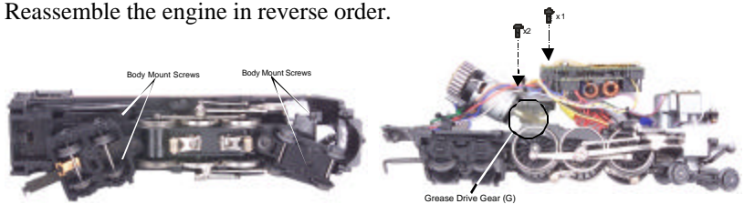
Figure 3. Greasing Points on the Engine and Body Mounting Screws
