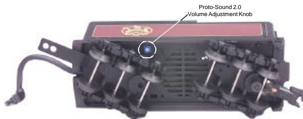
Figure 1. Adjusting the Proto-Sound 2.0 Volume Level
