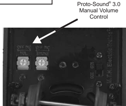
Figure 7: Manual Volume Control
