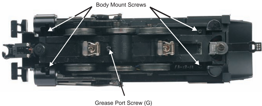
Fig. 9 and 10: Grease Points and Removing the Body
