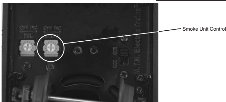
Fig. 3: Smoke Unit Control
