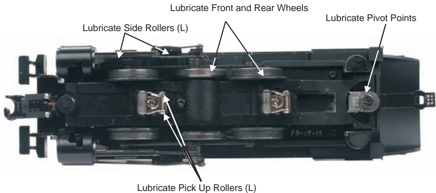
Fig. 1: Lubricating the Locomotive
