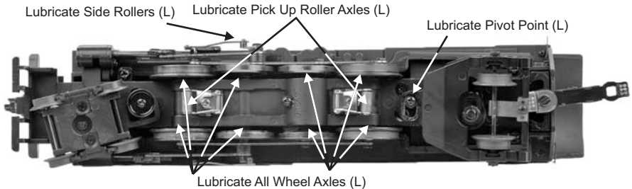
Figure 7: Lubricating the Locomotive
