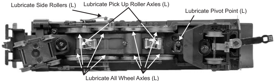
Fig. 1: Lubricating the Locomotive
