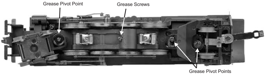
Figure 8: Grease Points
