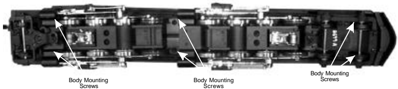
Figure 10: Removing The Boiler From The Chassis
