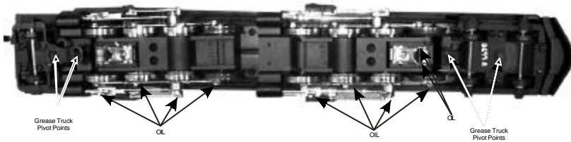
Figure 8: Lubricating The Locomotive Chassis
