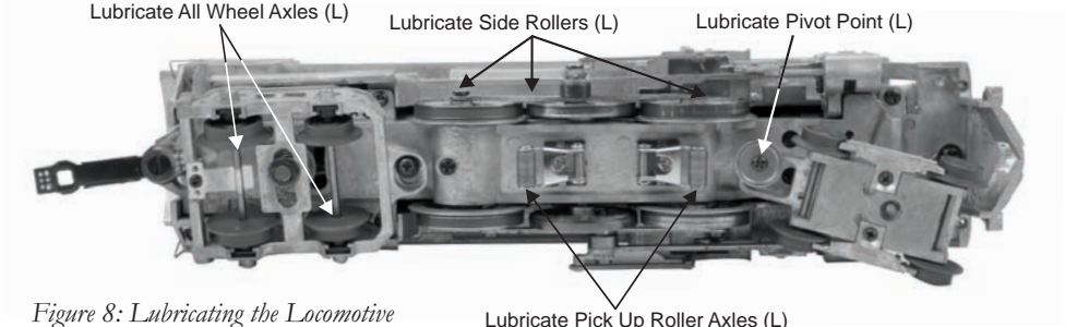
Figure 8: Lubricating the Locomotive
