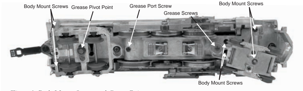
Figure 9: Body Mount Screws and Grease Points
