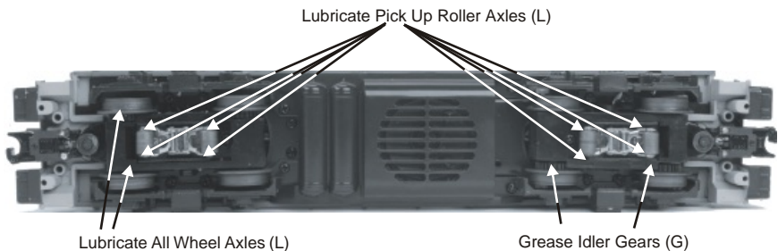
Figure 5: Lubrication Points
