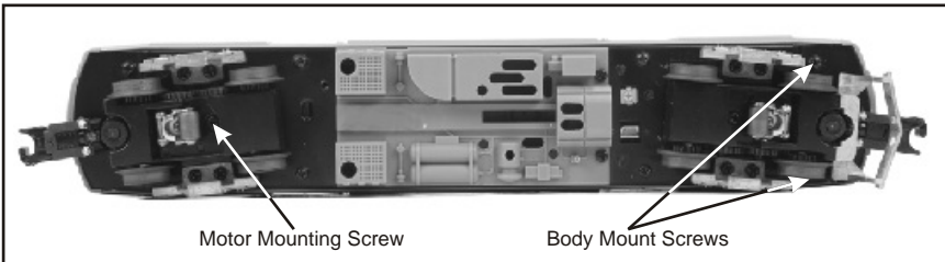
Figure 4. Body Removal Screw Locations
