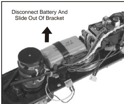
Figure 8. Battery Location.
