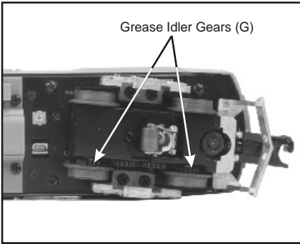
Figure 5. Greasing The Idler Gears
