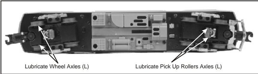
Figure 3. Lubrication Points on the Locomotive.
