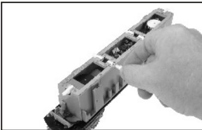
Figure 6. Replacing the Light Bulbs
