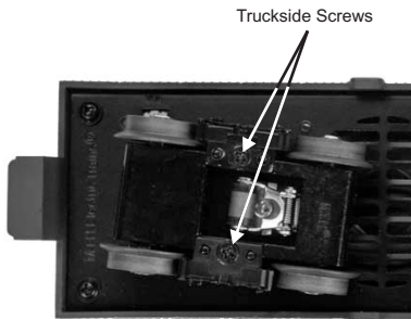
Figure 6: Truckside Screws
