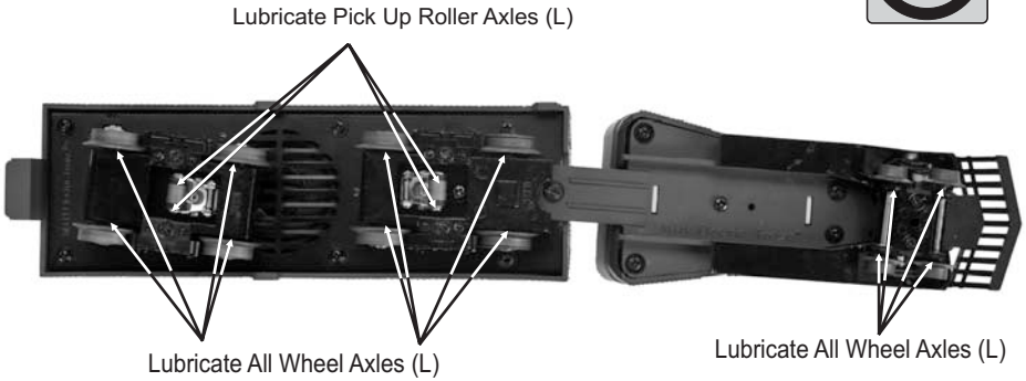
Figure 4: Lubrication Points on the Locomotive
