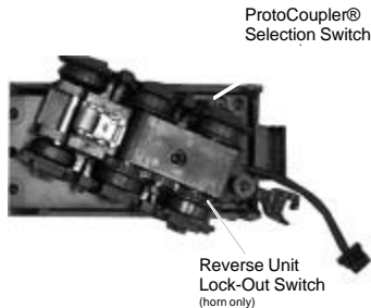
Figure 1: Lock-Out Switch Location
