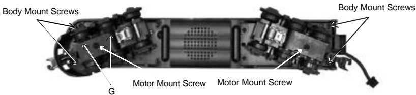
Figure 7: Lubricate The Locomotive Chassis Trucks
