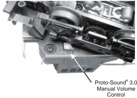
Figure 3: Manual Volume Control
