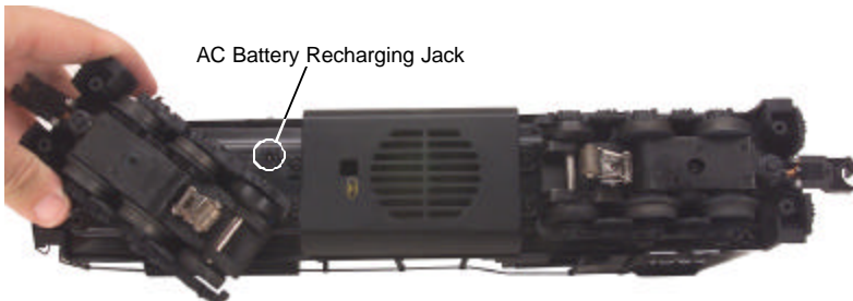
Figure 6. Replacing the Battery. Location of the Battery Re-charging Jack.
