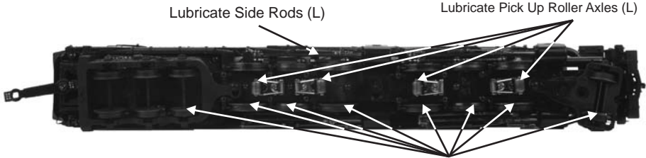
Fig. 9: Lubricating the Locomotive
