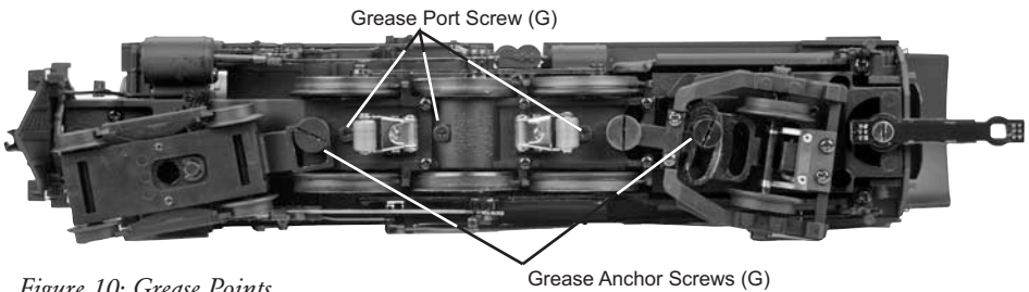
Figure 10: Grease Points
