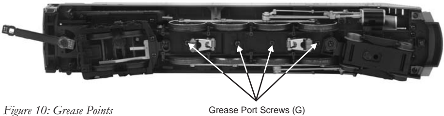
Figure 10: Grease Points
