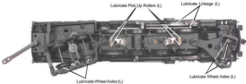
Figure 5: Lubrication Points
