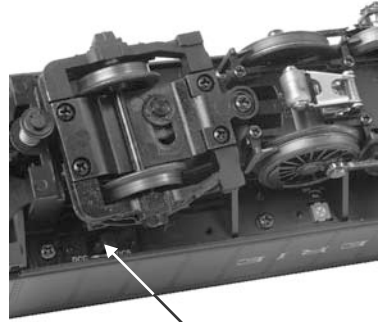
DCS/DCC Switch
