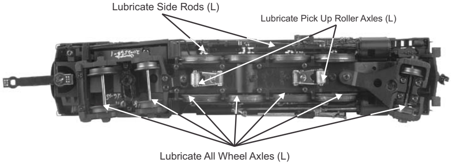
Fig. 9: Lubricating the Locomotive
