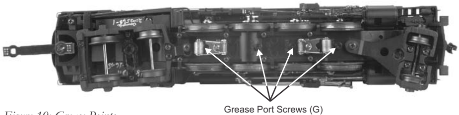
Figure 10: Grease Points
