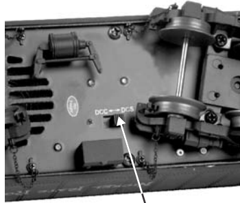
DCS/DCC Switch
