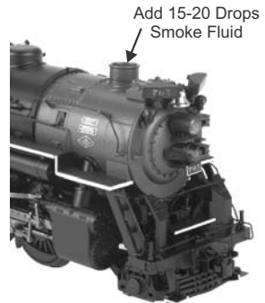
Figure 12: Adding Fluid
