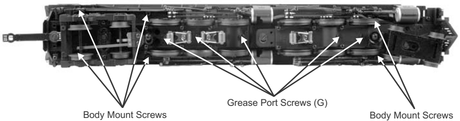
Figure: Grease Points / Body Mount Screws
