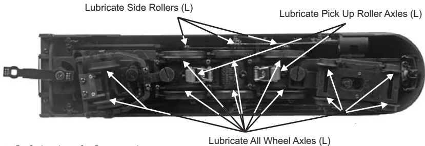
Fig. 1: Lubricating the Locomotive
