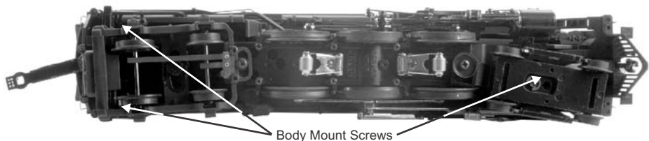
Figure: Removing the Body
