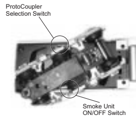
Figure 1: Locating The Smoke Unit & ProtoCoupler Selection Switch
