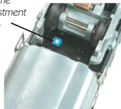
Figure 1 - Proto-Sound 2.0 Volume Adjustment Knob
