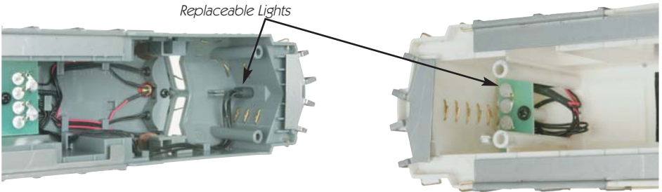
Figure 6 - Replacing the Headlights
