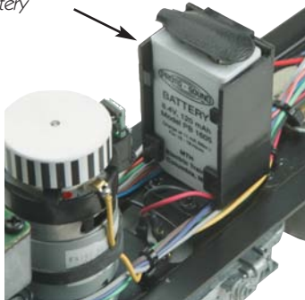
Figure 9- Replacing the Battery
