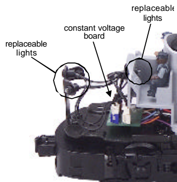
Figure 9. Locations of Replacable Lights
