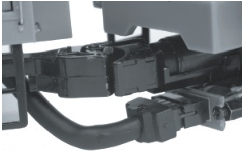
Correct way to Connect wire harness plug into the receptacle
