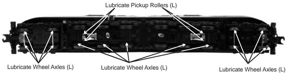
Figure 6. Lubrication Points on the Locomotive
