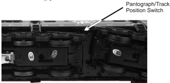
Figure 4: Pantograph/Track Position Switch
