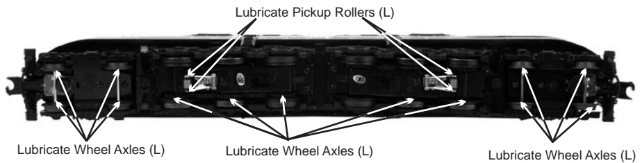
Figure 1. Lubrication Points on the Locomotive
