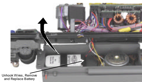
Figure 10: Removing The Battery Located In The Fuel Tank (4 Screws)
