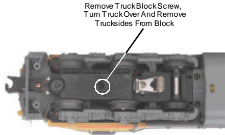
Figure 7: Removing The Truck Block To Access Trusside Screws
