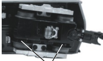
Grease Idler Gears (G)
