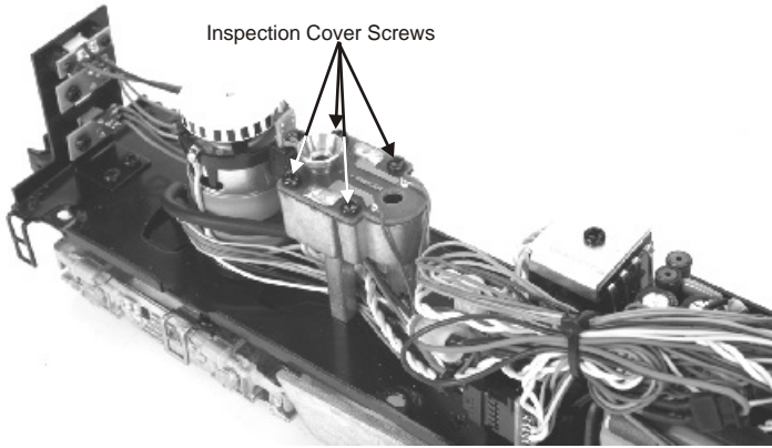
Figure 11. Inspecting the Smoke Unit Wick
