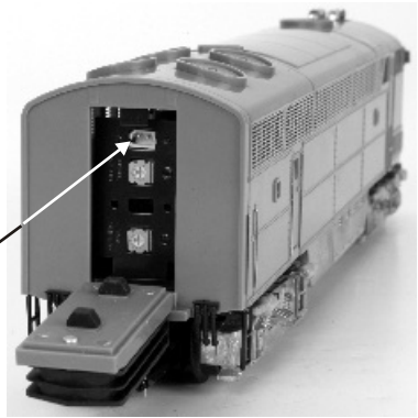
Figure 9. Battery Charger Port location.
