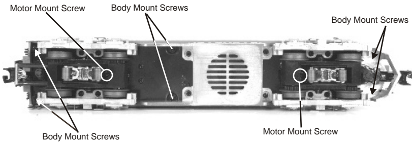
Figure 6. Body Removal Screw Locations
