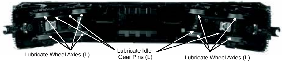
Figure 1. Lubrication Points on the Locomotive
