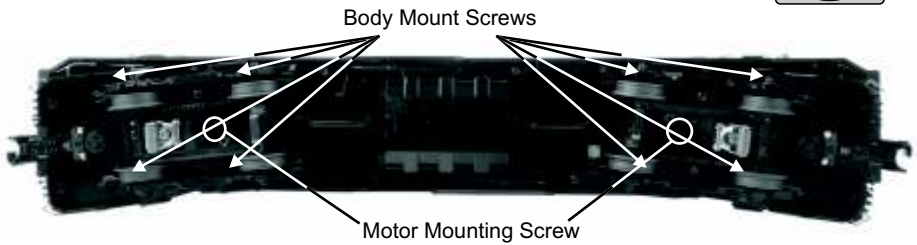
Figure 9: Body Removal Screw Locations and Motor Mounting Screws
