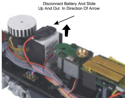
Figure 9: Removing The Battery
