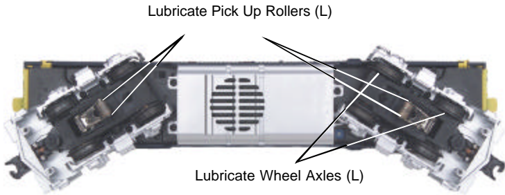
Figure 1. Lubrication Points on the Locomotive
