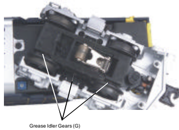
Figure 6: Greasing The Idler Gears
