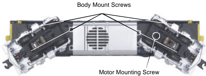
Figure 5: Body Removal Screw Locations
