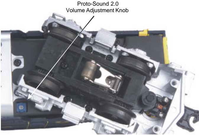
Figure 4: Manual Volume Adjustment Knob
