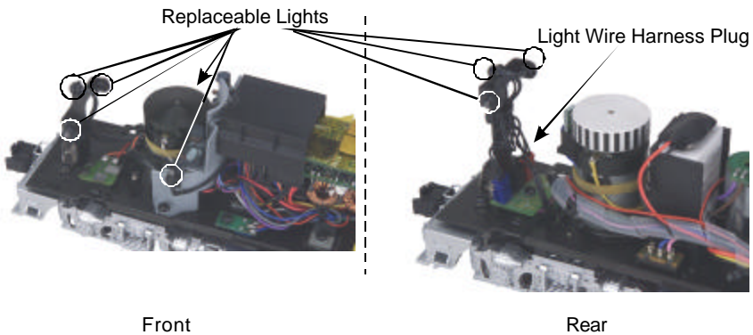
Figure 7: Removing The Replaceable Lights
