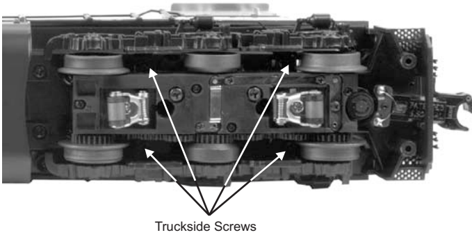
Figure: Truckside Screws
