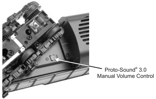
Figure: Manual Volume Control
