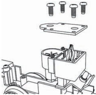
Smoke Unit Cover
