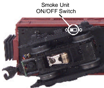
Figure 4. Smoke Unit ON/OFF Switch
