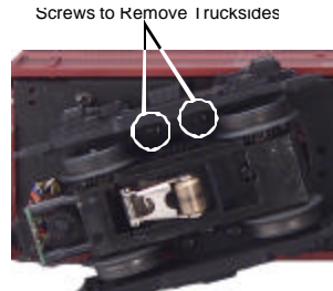
Figure 8. Locations of Truckside Mounting Screws
