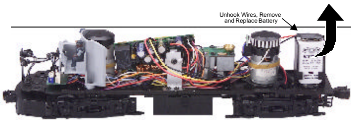
Figure 10. Replacing the Battery
