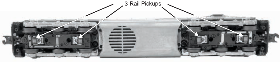
Figure 4: 3-Rail Pickups
