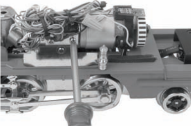
Fig. 11: Unscrewing Gearbox screws
