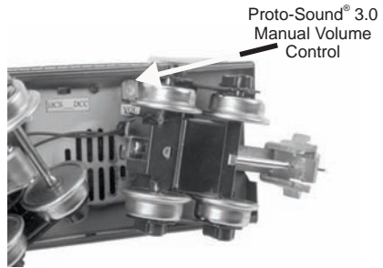
Figure 7: Manual Volume Control
