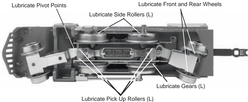
Fig. 1: Lubricating the Locomotive
