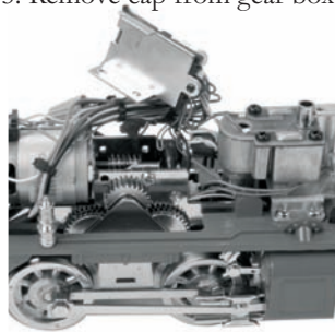
Fig. 12: Removing Cap
