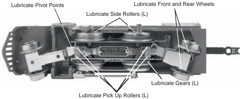
Fig. 8: Lubricating the Locomotive
