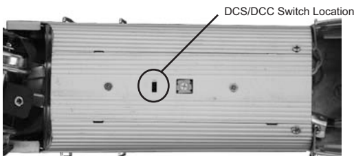
Figure 6: Changing from DCS to DCC Mode
