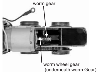
Figure 12: Grease Worm Gear
