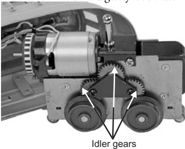
Figure 11: Grease Idler Gears
