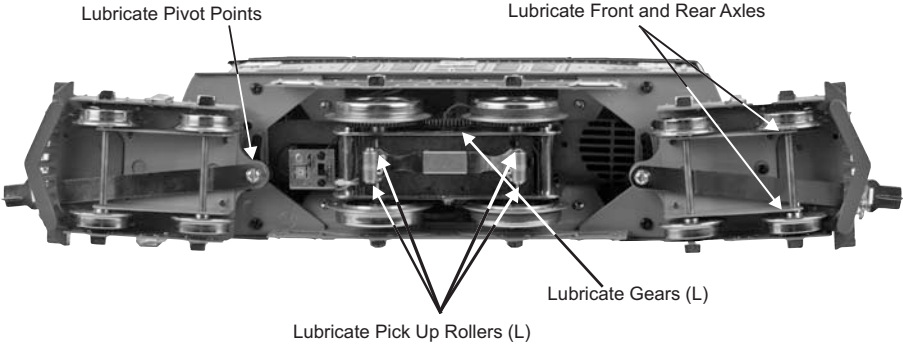
Fig. 5: Lubricating the Locomotive
