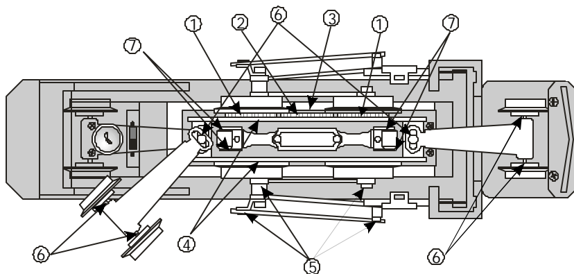
Figure 7: Lubricating The Locomotive Chassis
