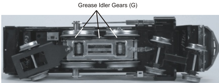
Greasing the Idler Gears
