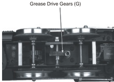
Greasing the gears
