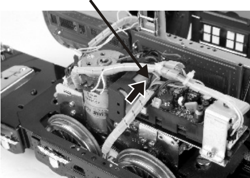
Figure 6. Battery Location.
