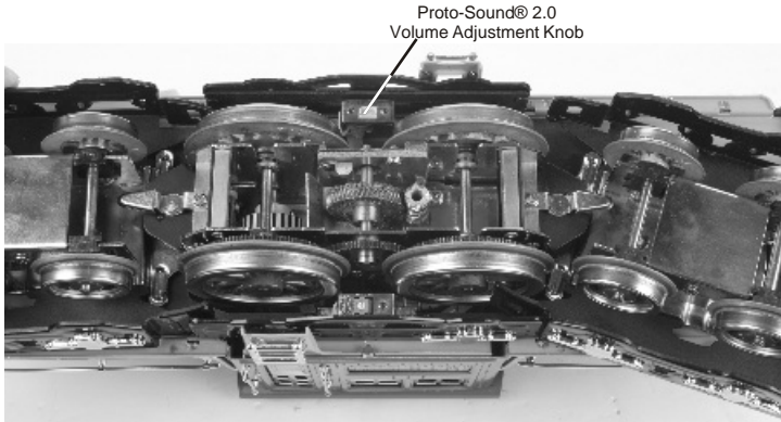
Figure 2. Manual Proto-Sound® 2.0 Volume Adjustment
