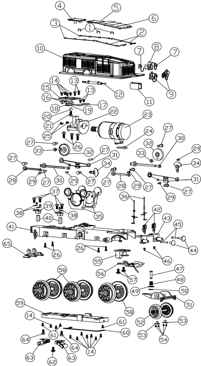
Crocodile Electric Engine Chassis(Right)
