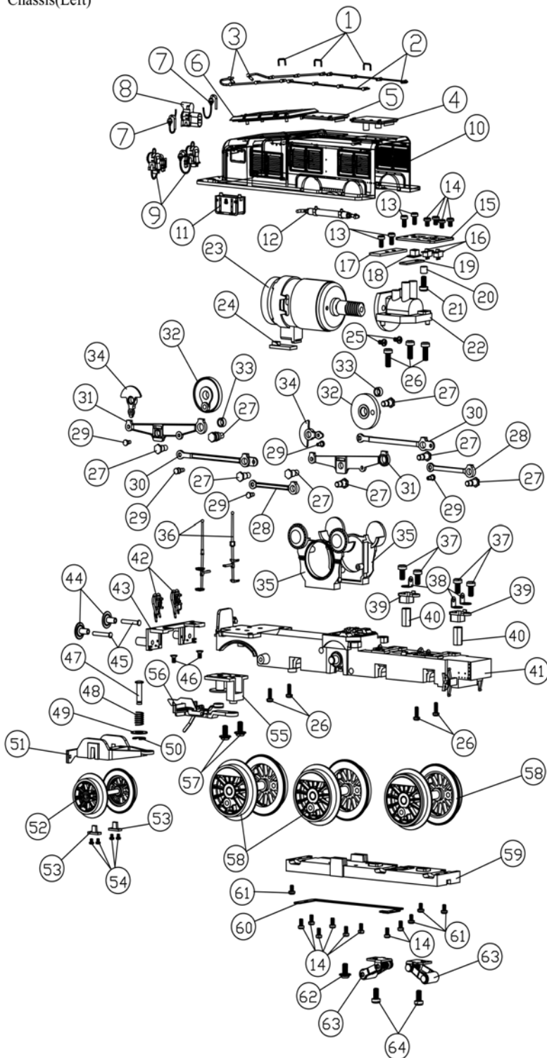
Crocodile Electric Engine Chassis(Left)
